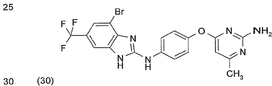
[4-(2-Amino-6-methyl-pyrimidin-4-yloxy)-phenyl]-[4-brom-6-trifluormethyl-1H-benzimidazol-2-yl]-amin
